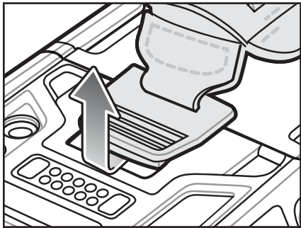
Figure 1-24 Remove Hand Strap Clip
