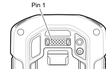
Figure A-1 I/O Connector
