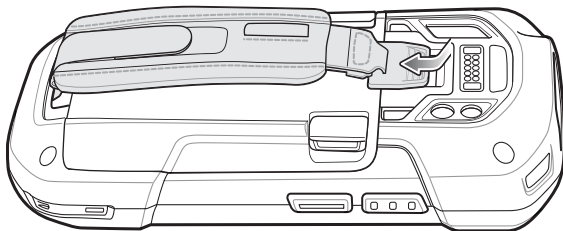
Figure 2-60 Secure Hand Strap Clip
