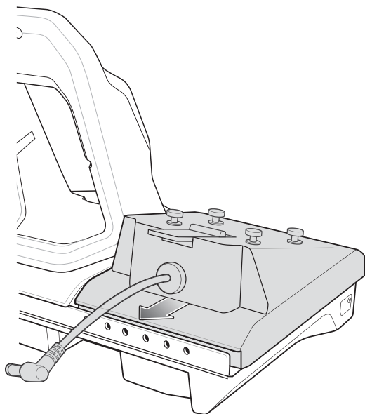
Figure 2-39 Install Adapter
