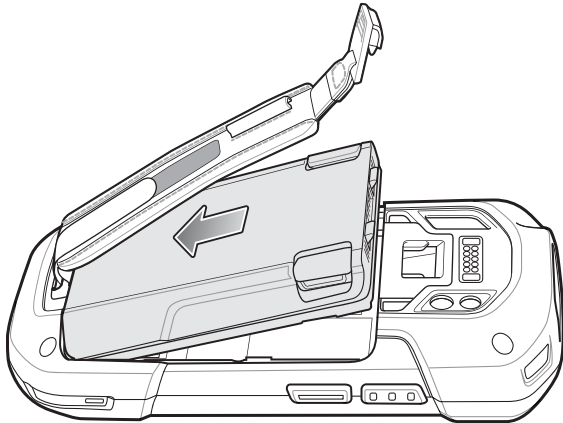
Figure 2-58 Insert Bottom of Battery into Battery Compartment
