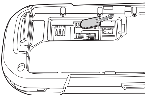
Figure 1-20 Remove Nano SIM Card
