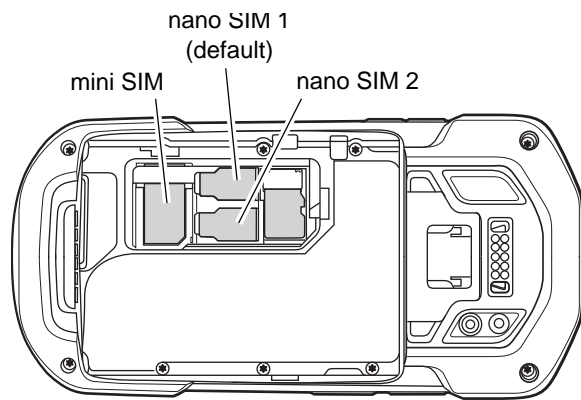
Figure 5-1 TC75x SIM Slot
