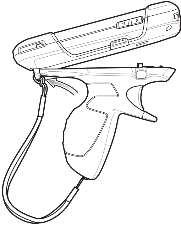
Figure 2-50 Connect Device to Trigger Handle
