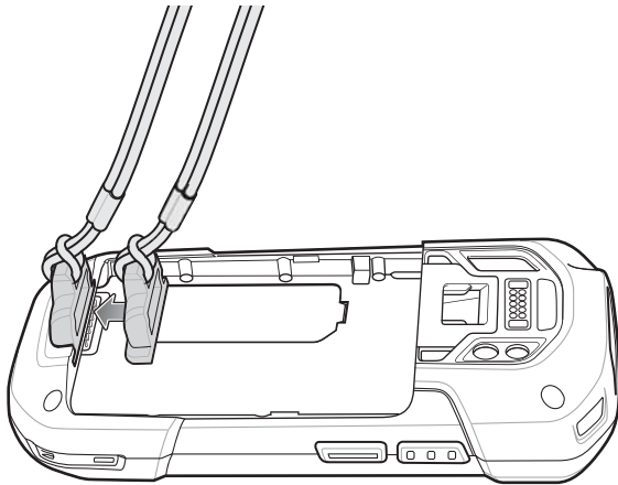
Figure 2-49 Insert Trigger Handle Plate
