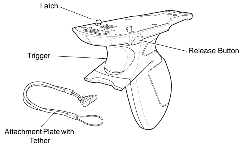
Figure 2-46 Trigger Handle
