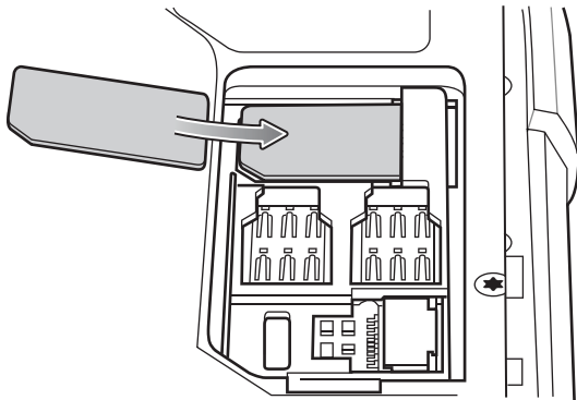
Figure 1-21 Insert Mini SIM/SAM Card
