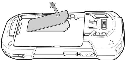
Figure 1-25 Remove Access Door
