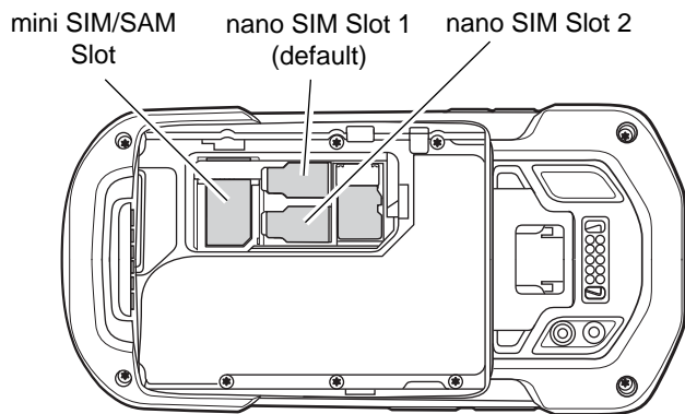
Figure 1-1 TC75x SIM Slot Locations
