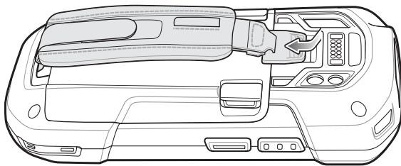
Figure 2-54 Remove Hand Strap Clip
