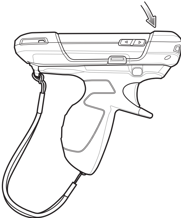
Figure 2-51 Rotate Device onto Trigger Handle
