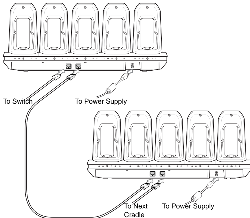
Figure 2-29 Daisy-chaining 5-Slot Ethernet Cradles
